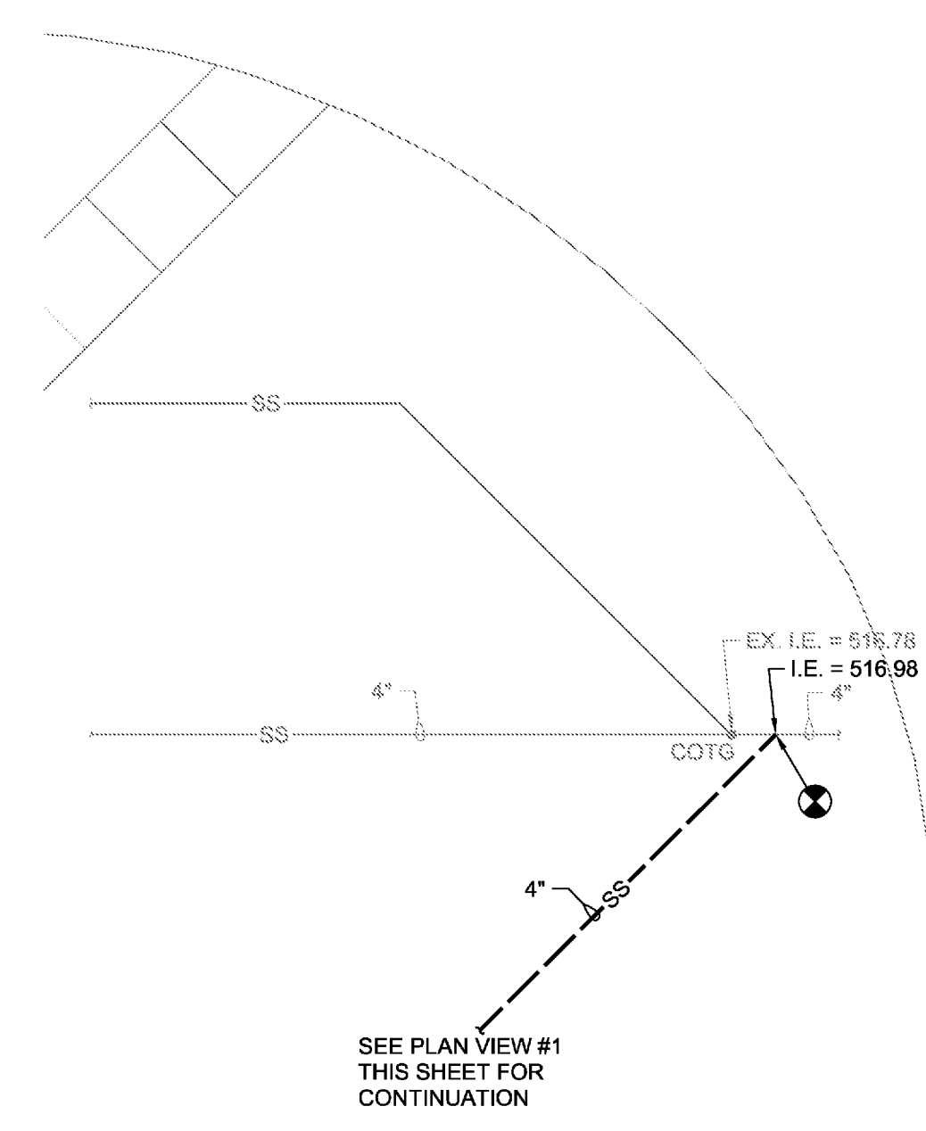
3 PARTIAL SITE PLAN - PLUMBING 1/8" = 1'-0"
