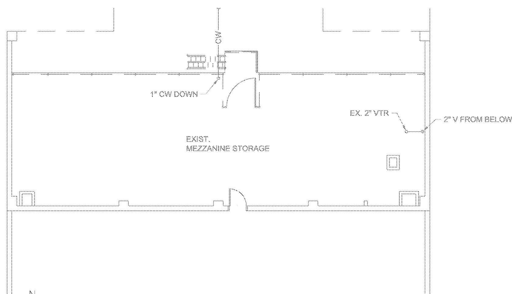
2 DEMOLITION MEZZANINE PLAN - PLUMBING 1/8" = 1'-0"
