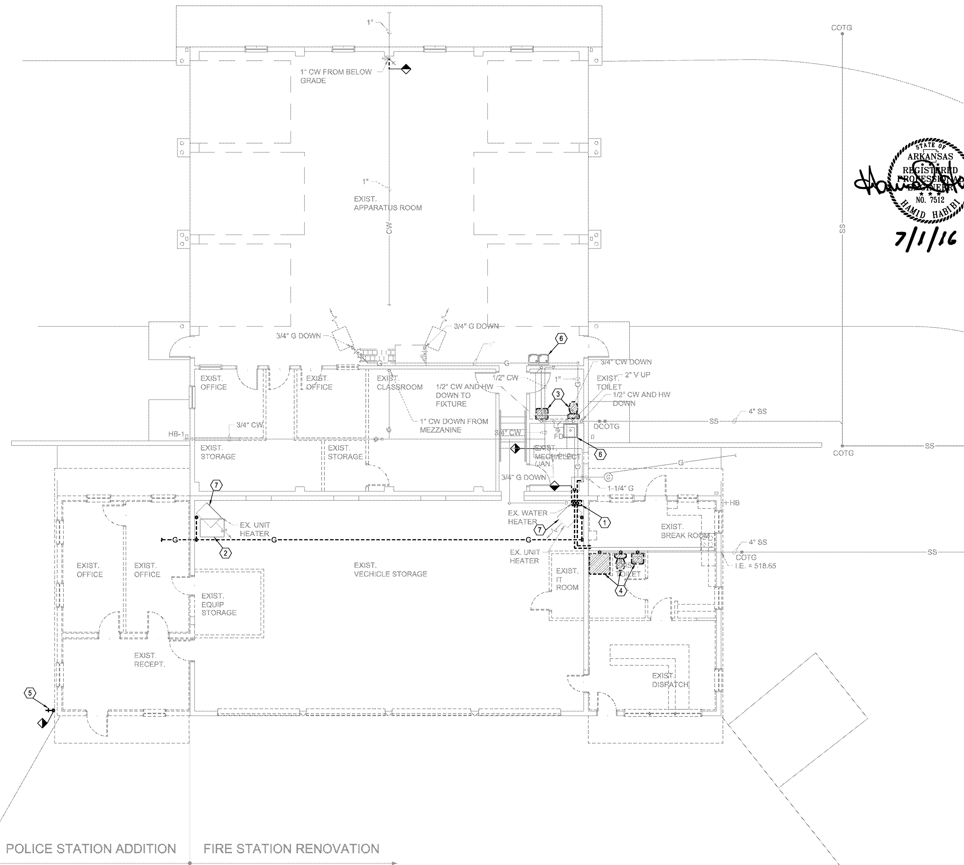
1 DEMOLITION FLOOR PLAN - PLUMBING 1/8" = 1'-0"
