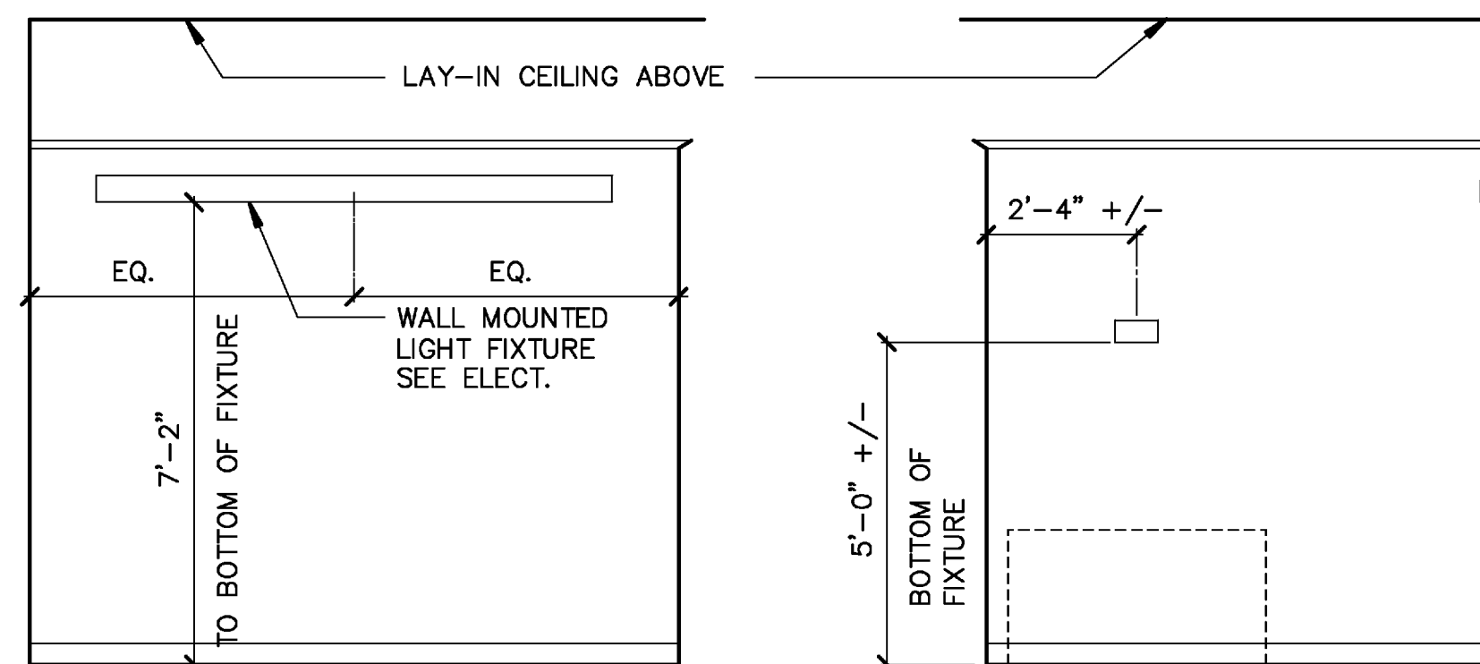
6 INTERIOR ELEV. SLEEPING QUARTERS #121 3/8" = 1'-0"
