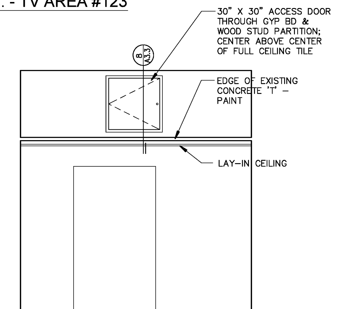
10 INTERIOR ELEV. - FOOD STR. #128 3/8" = 1'-0"
