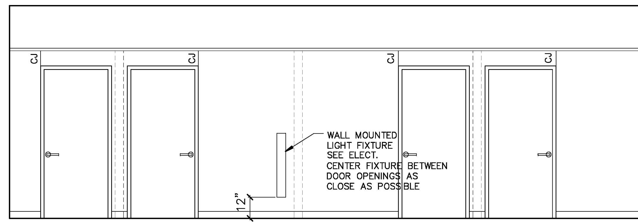
3 INTERIOR ELEV. - CORRIDOR #119 3/8" = 1'-0"
