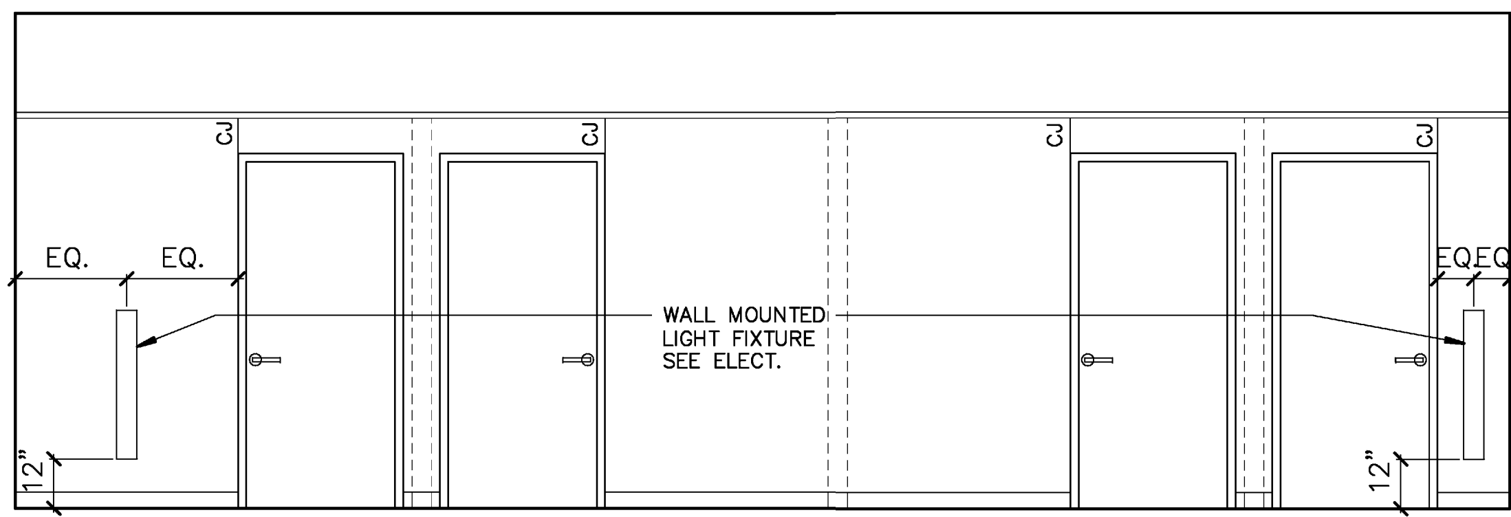
2 INTERIOR ELEV. - CORRIDOR #119 3/8" = 1'-0"
