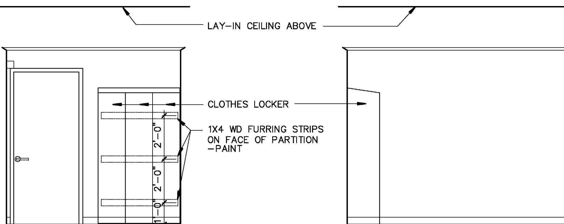
4 INTERIOR ELEV. SLEEPING QUARTERS #121 3/8" = 1'-0"
