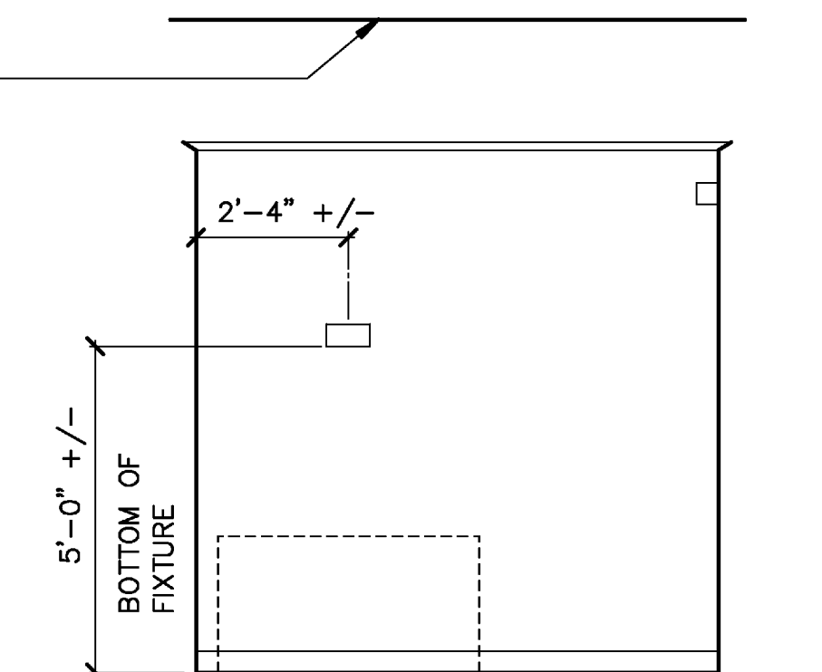
7 INTERIOR ELEV. SLEEPING QUARTERS #121 3/8" = 1'-0"
