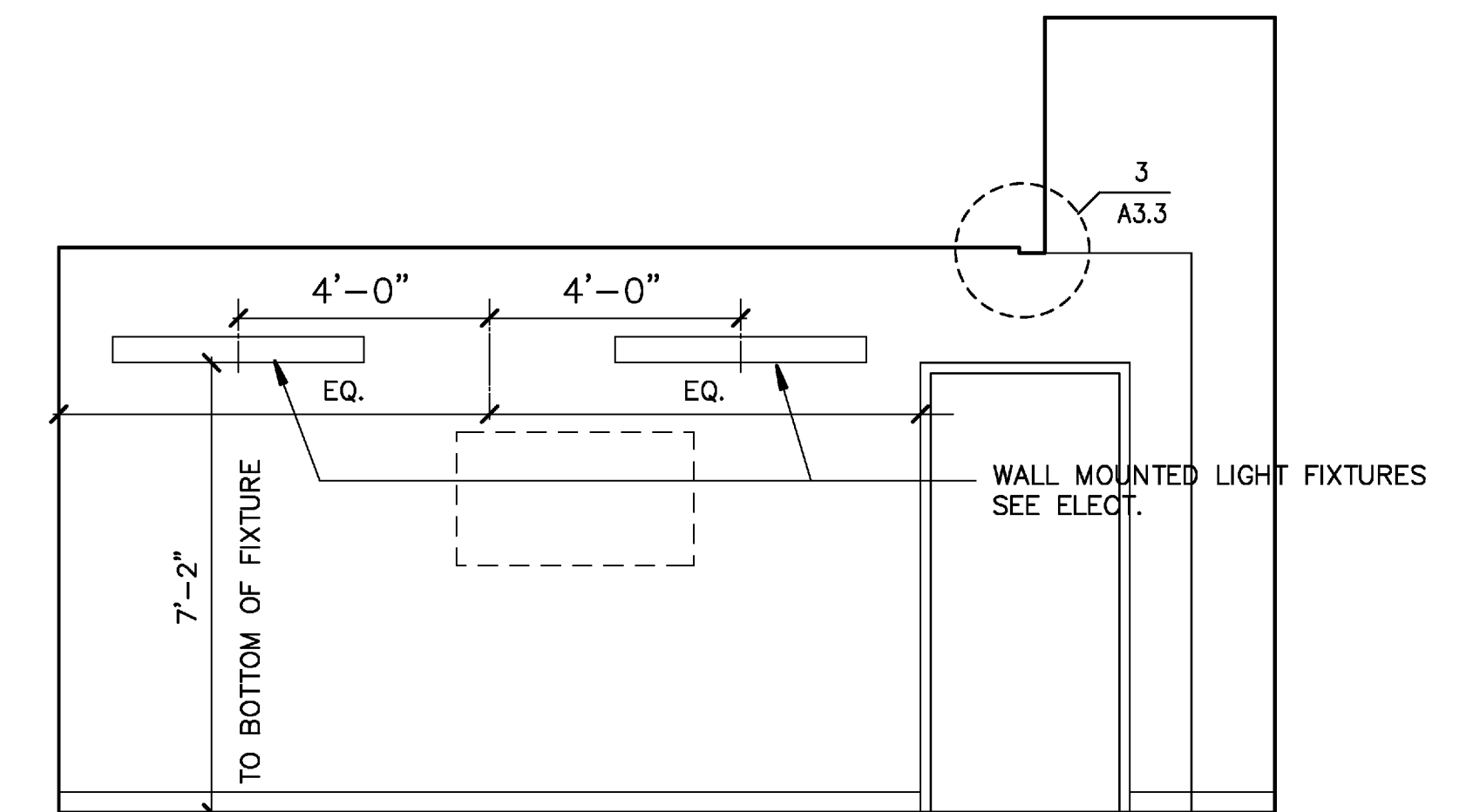
8 INTERIOR ELEV. - TV AREA #123 3/8" = 1'-0"
