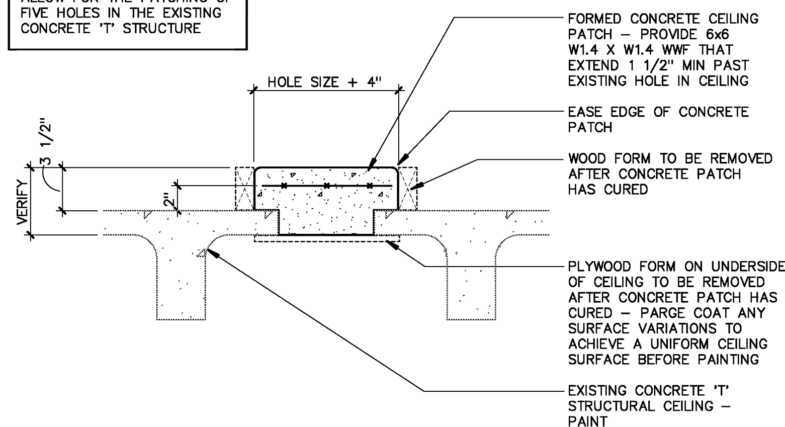
2 CEILING PATCH DETAIL 1 1/2" = 1'-0"
